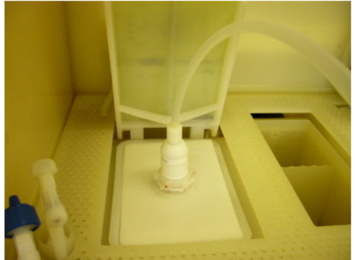
QC Dispense Head with Check Valve
