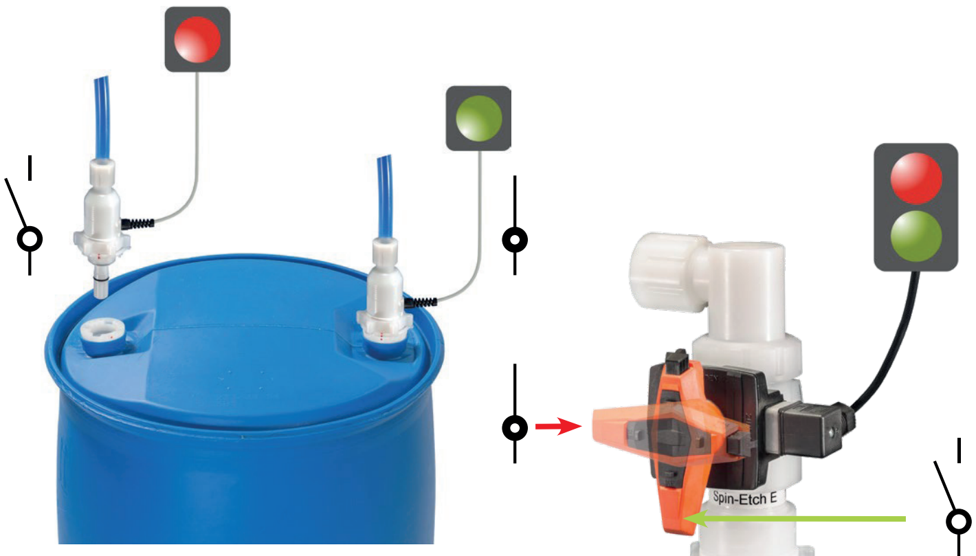
Signalling with full connection to dip tube
